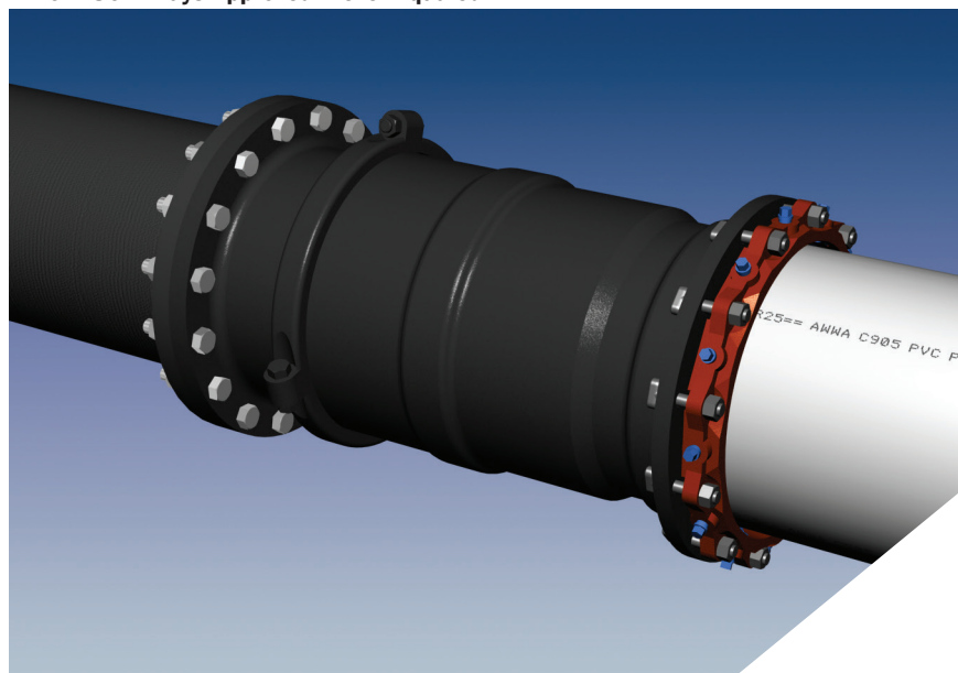
▲ Series 216C0 EX-TEND, 16 inch combination mechanical joint by flanged expansion joint. (DIP by PVC)
