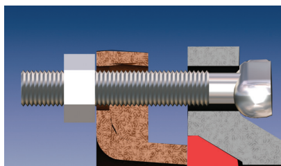
The EBAA-Seal deflects and compresses better to the MJ gasket recess than the SMJ gasket, generating greater sealing capabilities with less bolt torque values.
