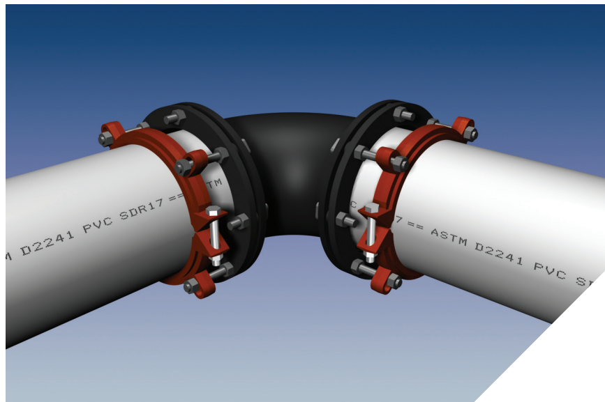
Series 65MJ12 restraining a mechanical joint fitting with a mechanical joint gland.
